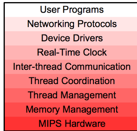
Figure 2: Layers of the Embedded Xinu kernel
